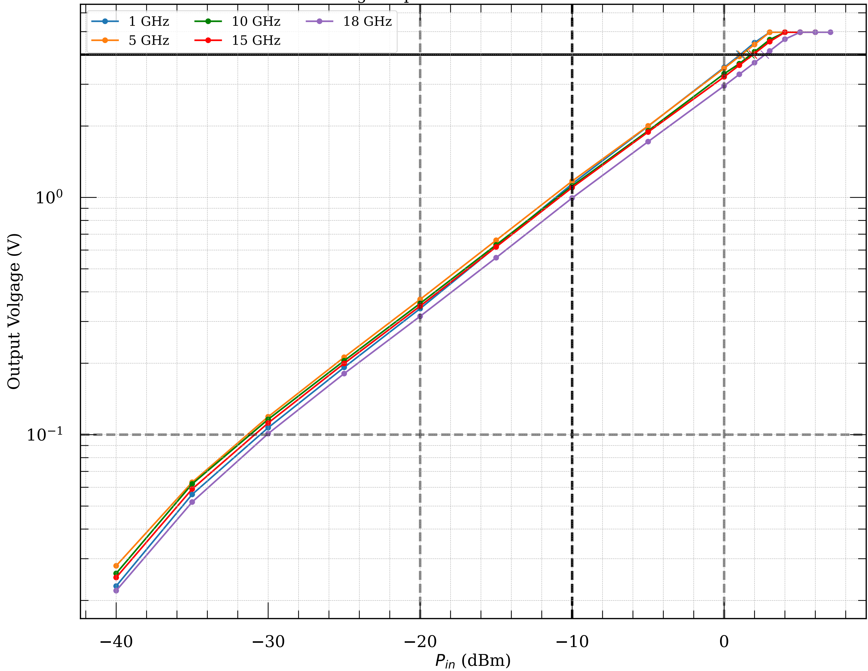
Measured voltage-to-power curve of detector module028v2
